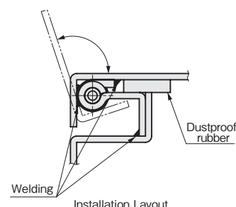
Installation Layout
