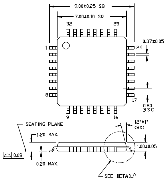
32-Lead Thin Plastic Quad Flatpack 7 x 7 x 1.0 mm A32 32-Lead Pb-Free Thin Plastic Quad Flatpack 7 x 7 x 1.0 mm A32
