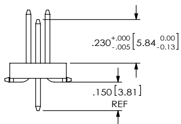
FIG 7 -TV: TRIPLE VERTICAL (DIFFERENT AS SHOWN, OTHERWISE SAME AS FIG 6) FOR EXISTING CUSTOMERS ONLY
