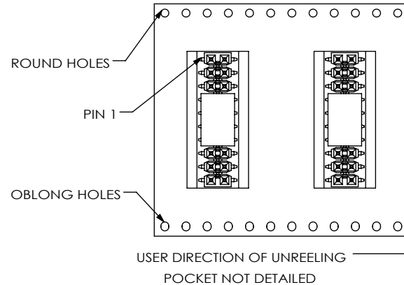
FIG 8 PACKAGING VIEWS
