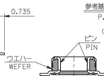
SECT.W-W(LOCK PART)
