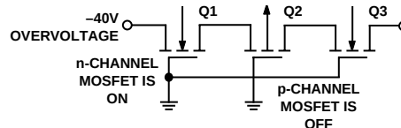
Figure 15. -40\text{ V} Overvoltage with Power OFF
