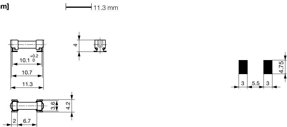
Soldering pads
