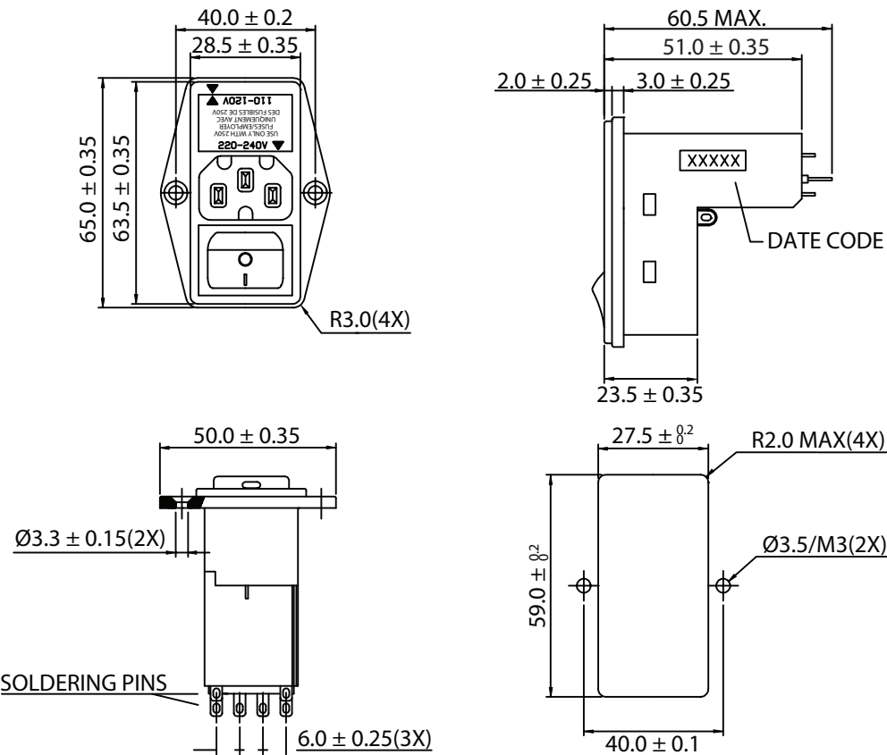
CUTOUT DIMENSION FOR SOCKET MOUNTING
