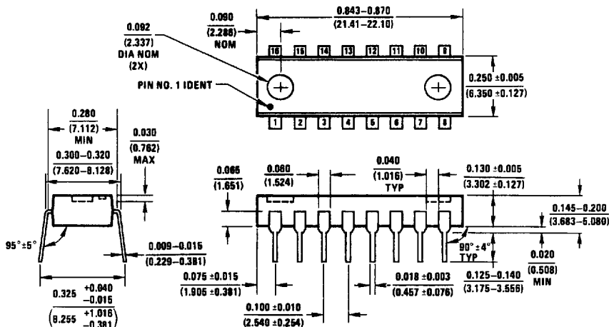
16-Lead (0.300" Wide) Molded Dual-In-Line Package Order Number LM1296N NS Package Number N16A
