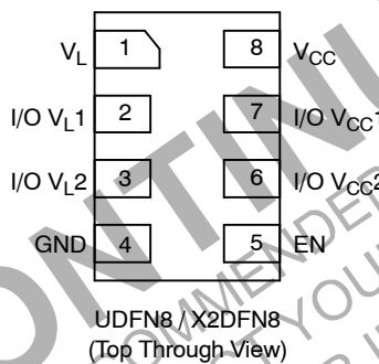
Figure 2. Pinout Diagram
