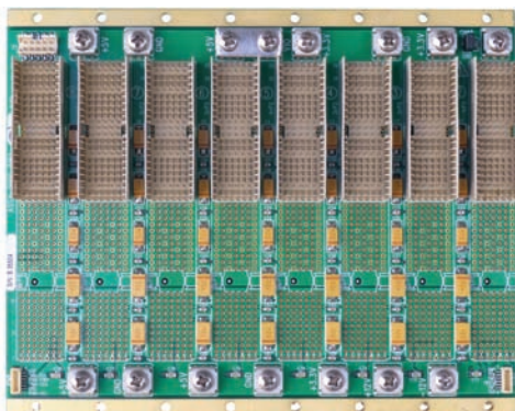
3U cPCI backplane with 8 slots, rear view
