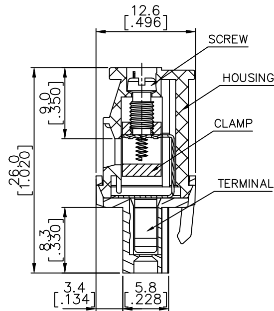
SECTION P-P
