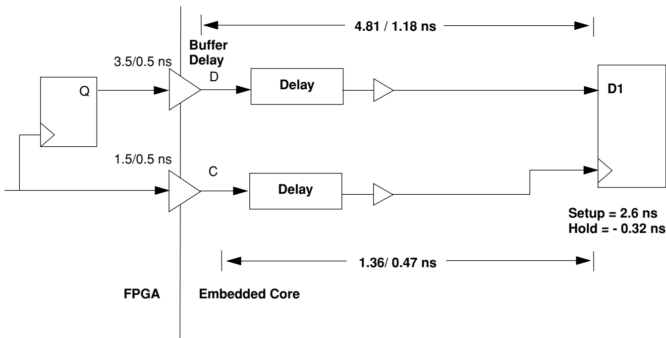
Figure 27. Data: SPI[A,B]_DATA/SOP/EOP/BE/ERR/PORT/WE/ADDR/SPI[A,B]_TXk_WD_CNT_RST /LINK_DIS
