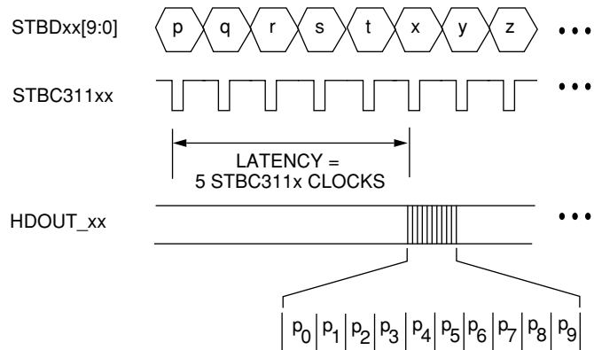
Figure 51. Transmit Path Timing - Single SERDES Channel (NOTE: xx = A, B, C, or D)
