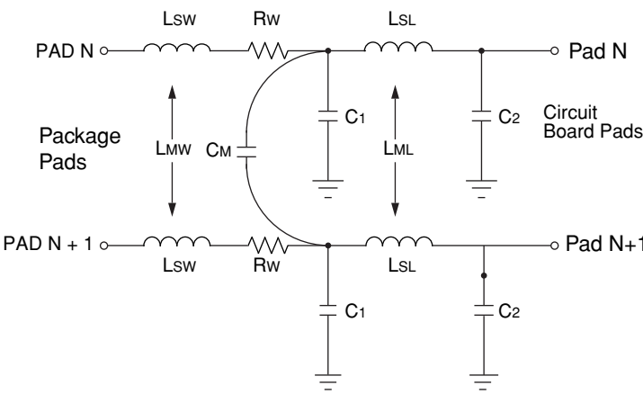
Figure 102. Package Parasitics
