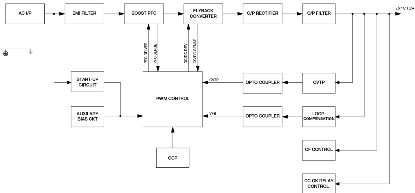
DRS-24V100W1□R
