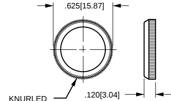
PLASTIC FACENUT (Wrench supplied N/C) .625" X .120" [15.87] X [3.04] BLACK - 384-17126-001 RED - 384-17126-002 WHITE - 384-17126-003
