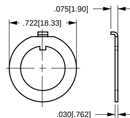
LOCKING RING ZINC - 728-15946 BLACK - 728-15947
