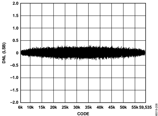
Figure 20. DNL Plot
