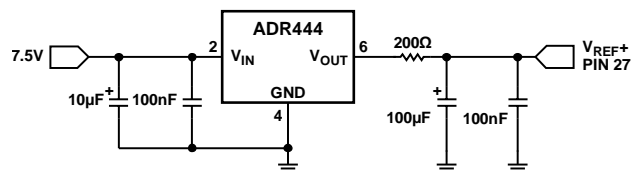
Figure 46. Reference Connection
