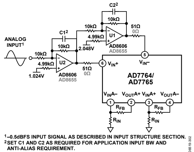
Figure 34. Driving the AD7765 Modulator Inputs Directly from a Single-Ended Source (On-Board Differential Amplifier Powered Down)
