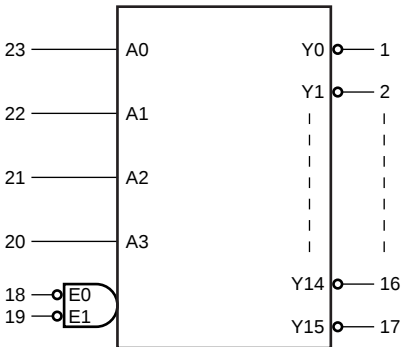
Fig 2. Logic symbol
