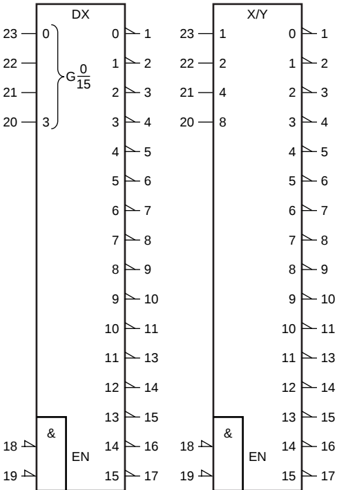
Fig 3. IEC logic symbol
