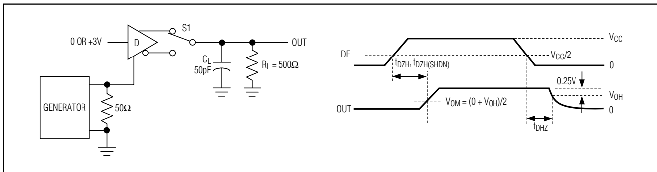
Figure 5. Driver Enable and Disable Times ( t_{DZH} , t_{DHZ} , t_{DZH(SHDN)} )
