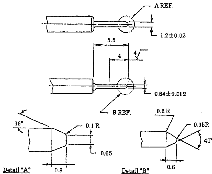
Fig. 6 Contact Insertion/Extraction Force Measuring Gage Design
