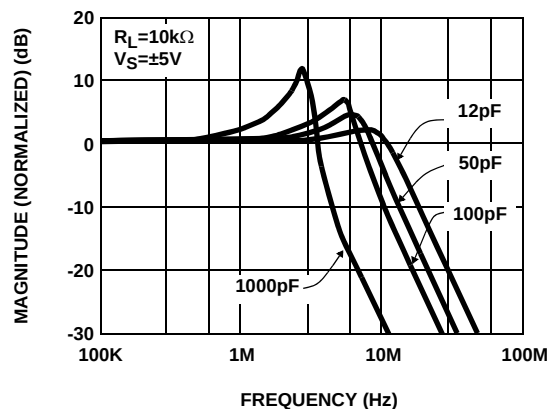
FIGURE 12. FREQUENCY RESPONSE FOR VARIOUS C_L
