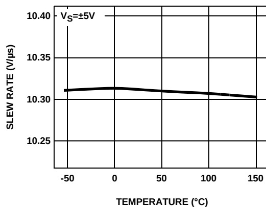
FIGURE 8. SLEW RATE vs TEMPERATURE
