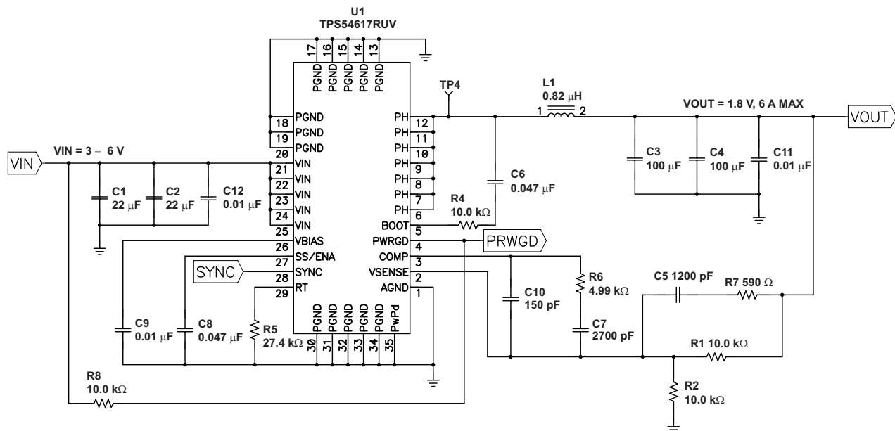
Figure 10. Application Circuit
