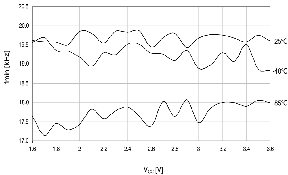
Figure 37-75.Maximum PDI frequency vs. V_{CC} .
