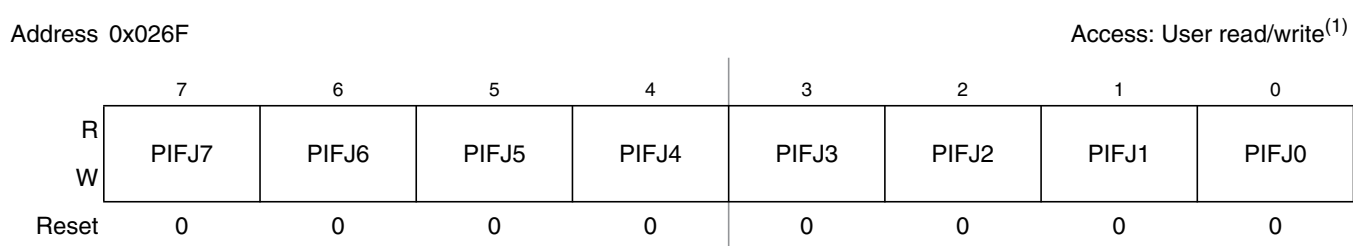
Figure 2-66. Port J Interrupt Flag Register (PIFJ)
