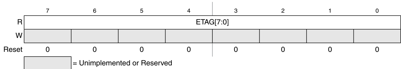
Figure 27-19. EEE Tag Counter Low Register (ETAGLO)
