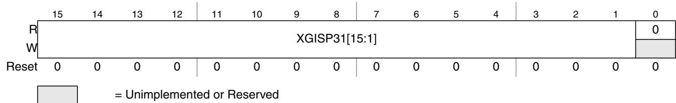
Figure 10-8. XGATE Initial Stack Pointer for Interrupt Priorities 3 to 1 (XGISP31)
