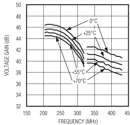
VHF HI VOLTAGE GAIN vs. FREQUENCY
