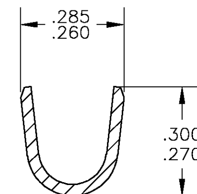
SECTION Y-Y
