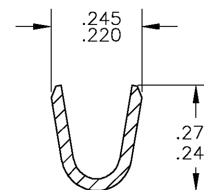
SECTION X-X
