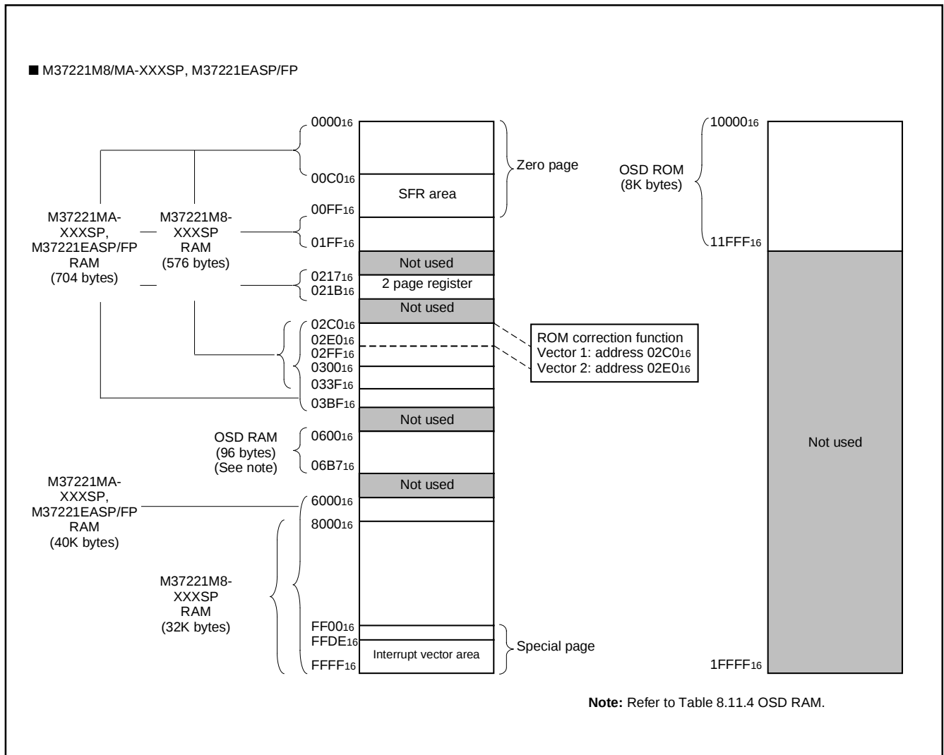
Fig. 8.2.2 Memory Map (M37221M8/MA-XXXSP, M37221EASP/FP)
