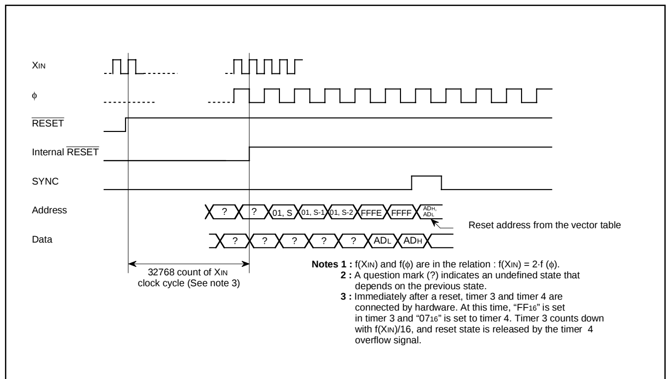
Fig. 8.13.2 Reset Sequence
