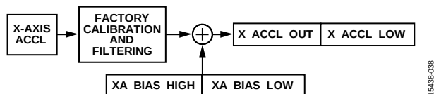
Figure 38. User Calibration Signal Path, Accelerometers
