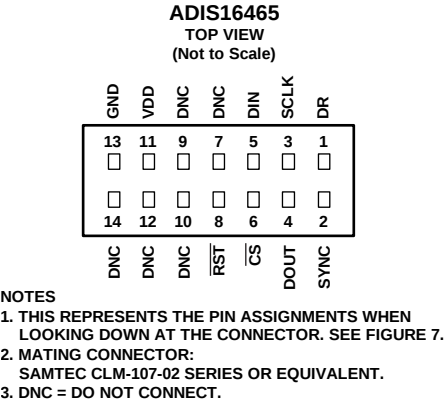
Figure 6. Pin Assignments, Bottom View
