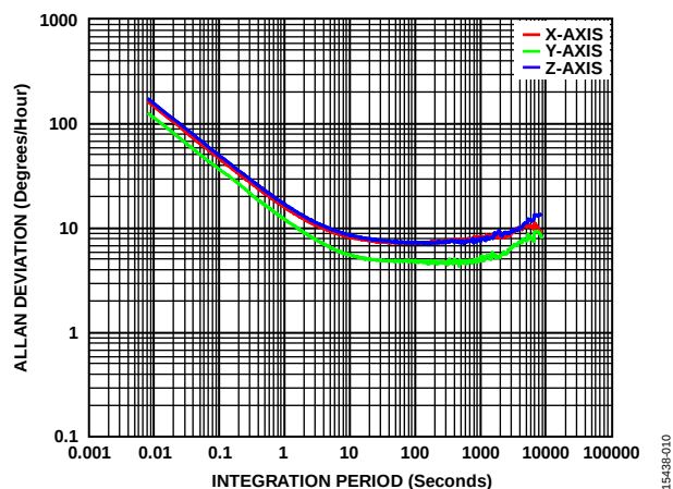
Figure 10. Gyroscope Allan Deviation, T_C = 25^\circ\text{C} , ADIS16465-3
