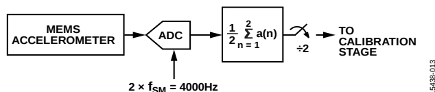
Figure 13. Accelerometer Data Sampling
