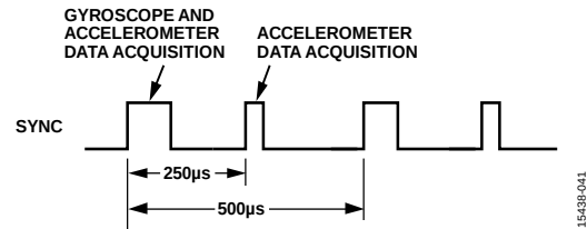
Figure 41. Sync Output Signal, Register MSC_CTRL, Bits[4:2] = 011
