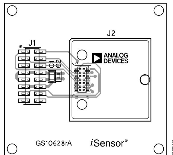
Figure 45. ADIS16IMU4/PCBZ Top View
