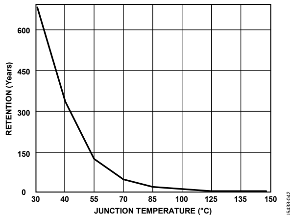
Figure 42. Flash Memory Retention
