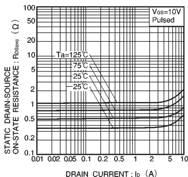
Fig.5 Static drain-source on-resistance vs. drain current
