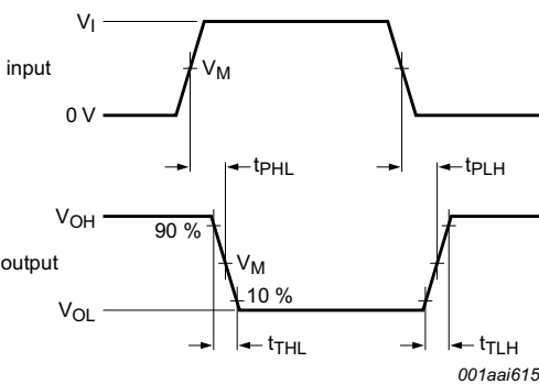
Fig 4. Input (nAn) to output (nȳn) propagation delays
