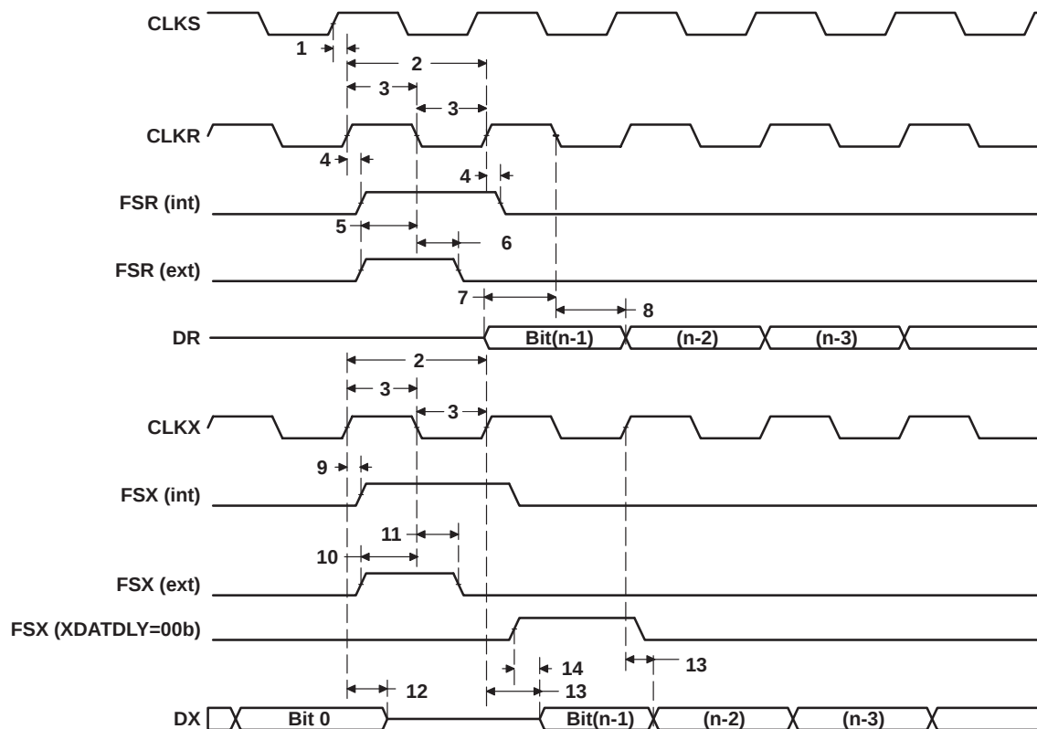
Figure 37. McBSP Timings
