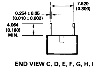
END VIEW C, D, E, F, G, H, I
