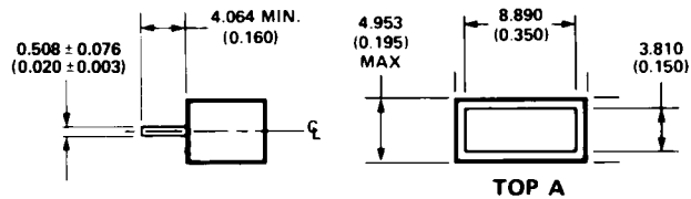
END VIEW A, B
