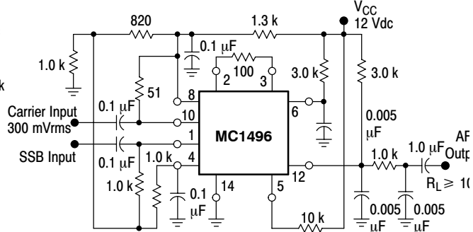
Figure 28. Product Detector (12 Vdc Single Supply)
