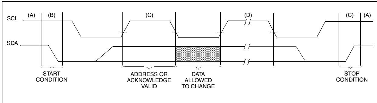
FIGURE 6-3: DATA TRANSFER SEQUENCE ON THE SERIAL BUS
