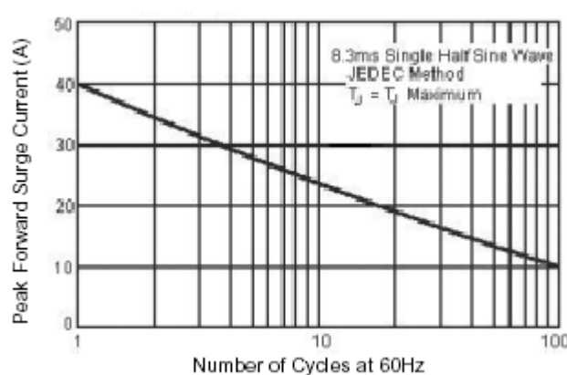
Maximum Non-Repetitive Peak Forward Surge Current
