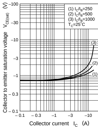
V_{CE(\text{sat})} - I_C
