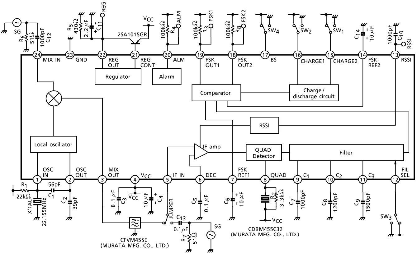
TEST CIRCUIT 1
