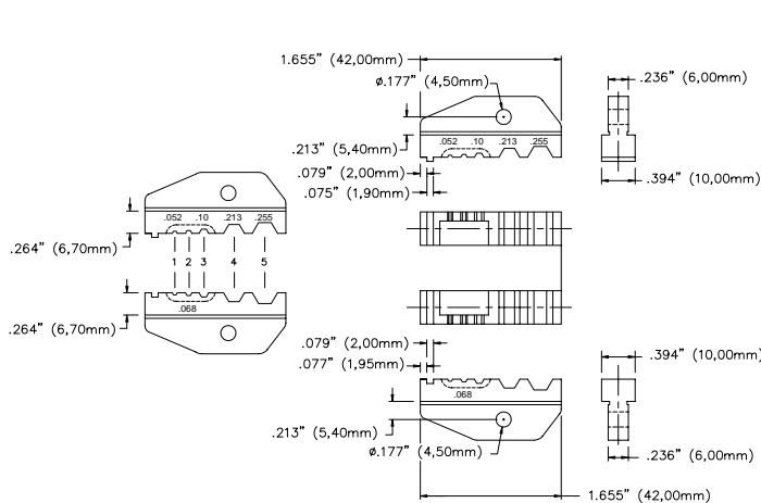
Model 7281 Crimp Die Set For Sizes .255/.213/.100/.068/.052
