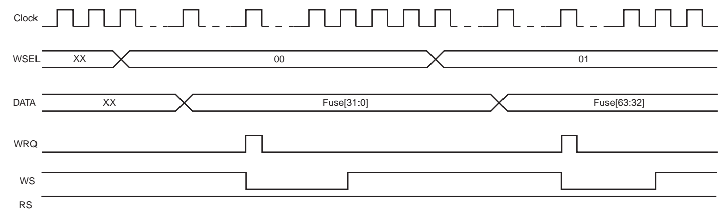
Figure 25-3. Fuse Write
