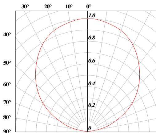
Radiation Pattern
