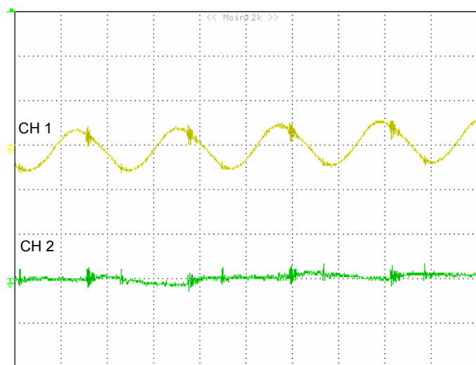
Figure 9: MGMT_PWR (3.3V) and BLUE_LED_PWR (5V) output ripple/noise (2μs/div):
