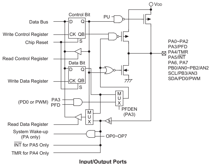
Input/Output Ports
