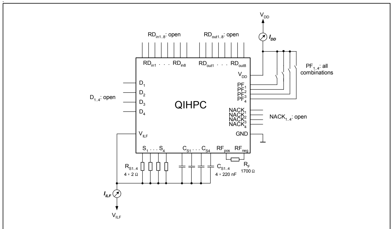
Figure 10 Supply Currents
