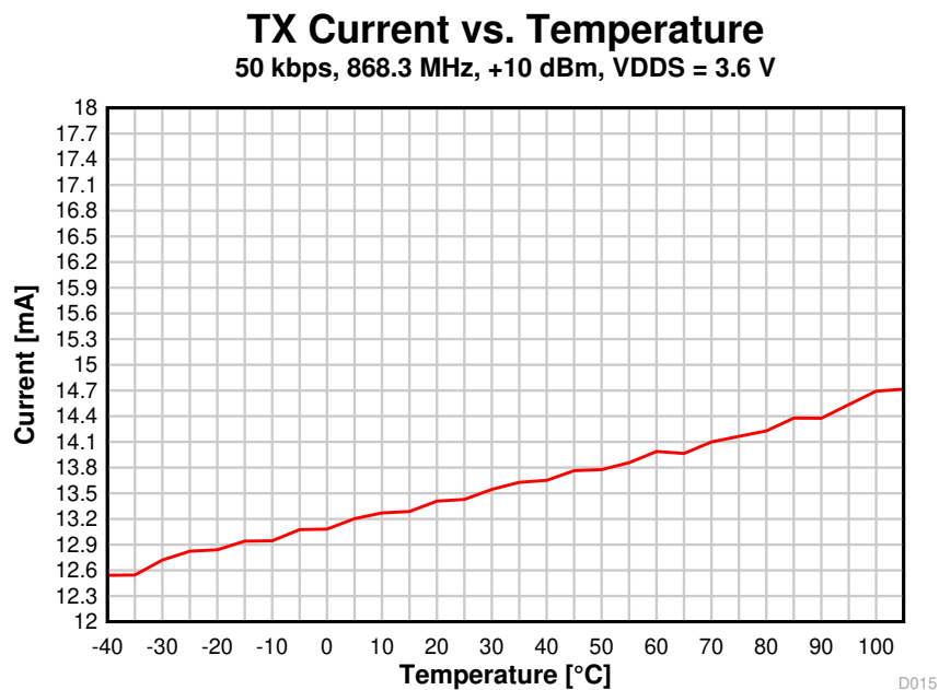
Figure 8-10. TX Current vs. Temperature (50 kbps, 868.3 MHz, VDD S = 3.6 V)
