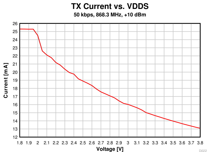
Figure 8-11. TX Current vs. Supply Voltage (VDD S ) (50 kbps, 868.3 MHz)
