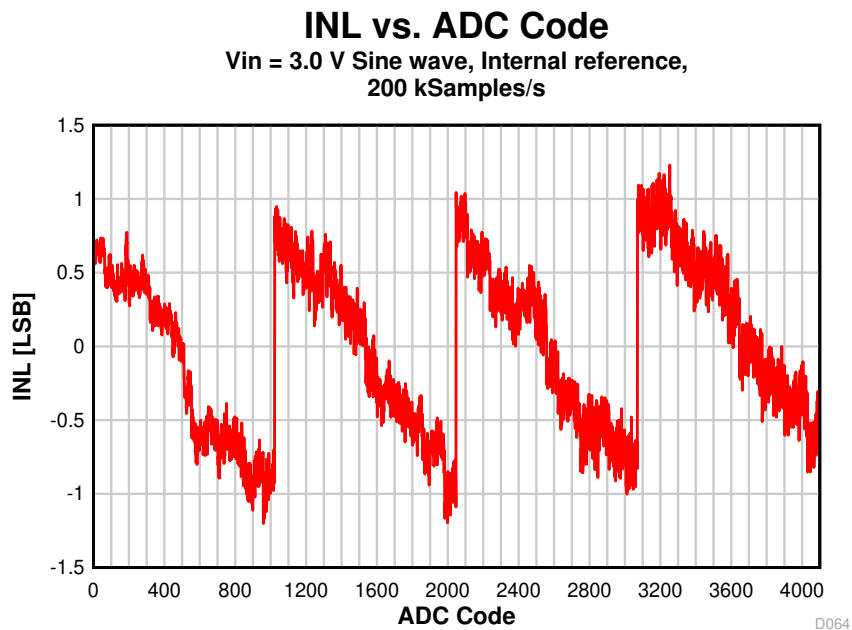
Figure 8-27. INL vs. ADC Code
