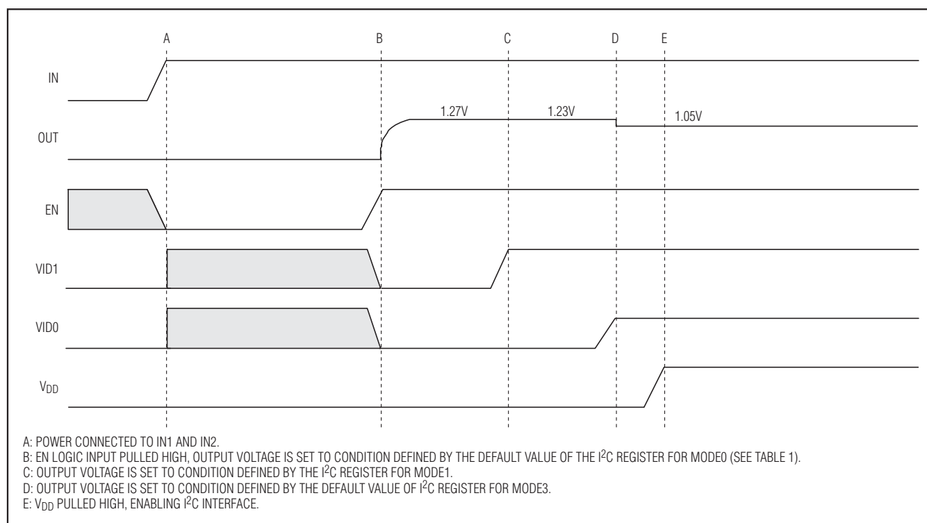
Figure 2. Power-Up Sequence
