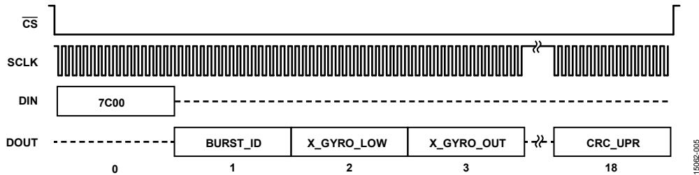
Figure 5. Burst Read Function Sequence Diagram, 19 Segments
