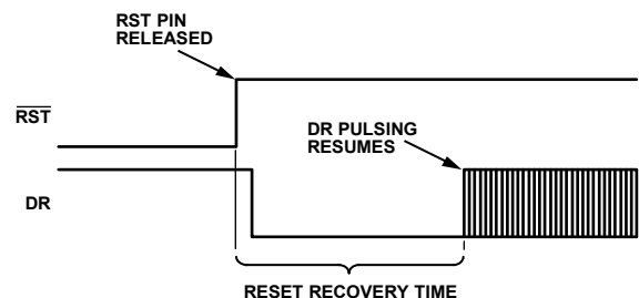
Figure 24. Data Ready Response During Reset ( \overline{RST} = 0 ) Recovery
