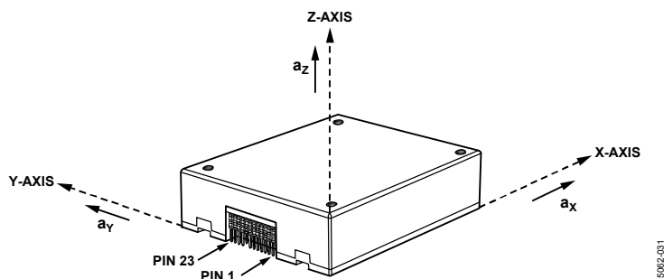
Figure 31. Accelerometer Axis and Polarity Assignments
