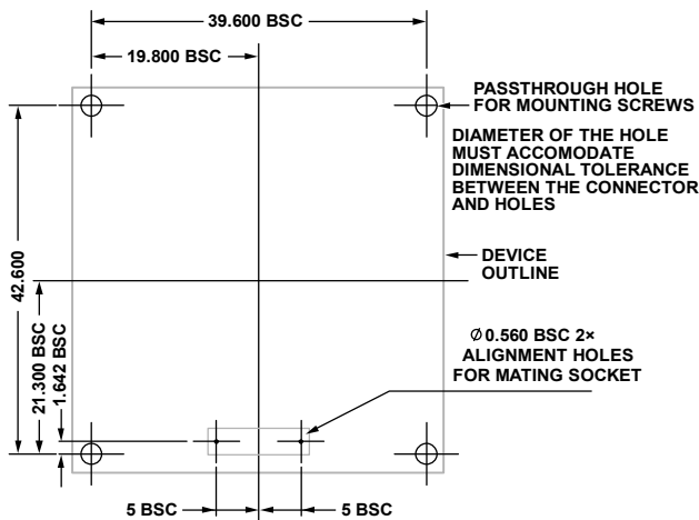
Figure 42. Suggested PCB Layout Pattern, Connector Down
