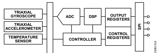
Figure 18. Basic Operation
