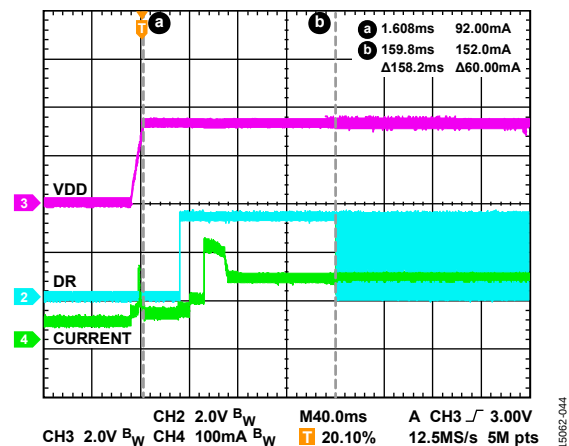
Figure 44. Transient Current Demand, Startup (DR Means Data Ready)
