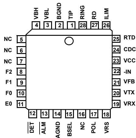
HC55184 (28 LD PLCC) TOP VIEW
