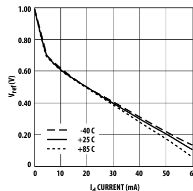
Figure 20. Control Voltage vs. Current and Temperature.
