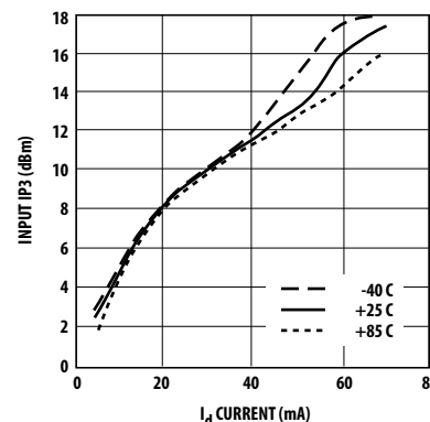
Figure 17. Input Third Intercept Point vs. Current and Temperature.
