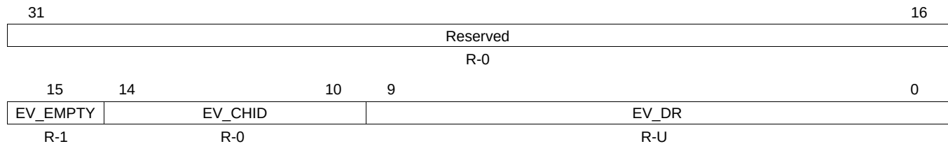
Figure 19-59. 10-bit ADC Event Group Results' FIFO Register (ADEVBUFFER) [offset = 90h-AFh]
