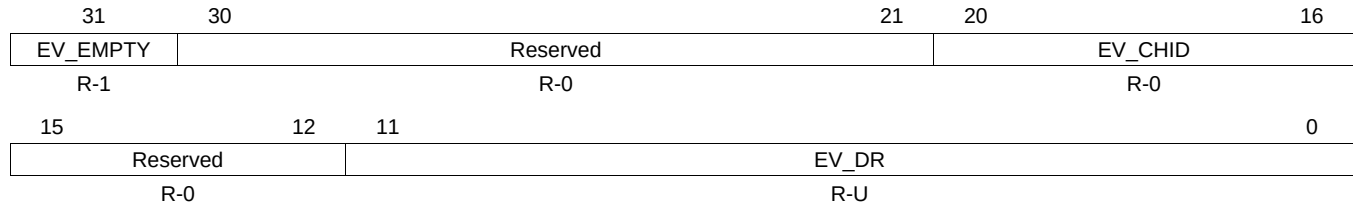
Figure 19-58. 12-bit ADC Event Group Results' FIFO Register (ADEVBUFFER) [offset = 90h-AFh]
