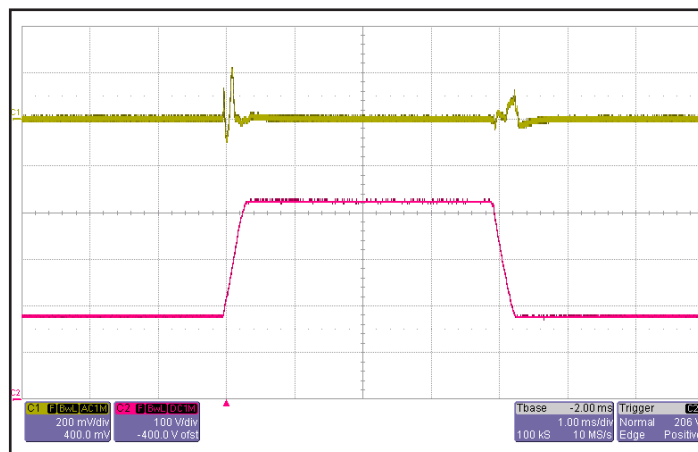
Figure 6: Output voltage response to step-change in input voltage (180V-425V-180V), at 60A load current. Load cap: 15μF tantalum capacitor and 1μF ceramic cap. Ch 1: V out (200mV/div), Ch 2: V in (100V/div).
