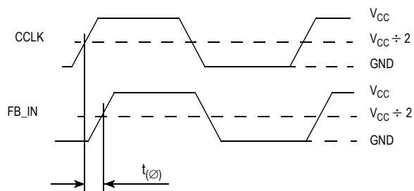
Figure 10. Propagation Delay ( t_{PD} , static phase offset) Test Reference
