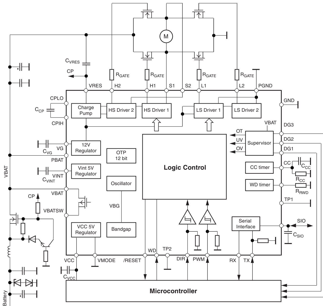
Figure 1. Block Diagram
